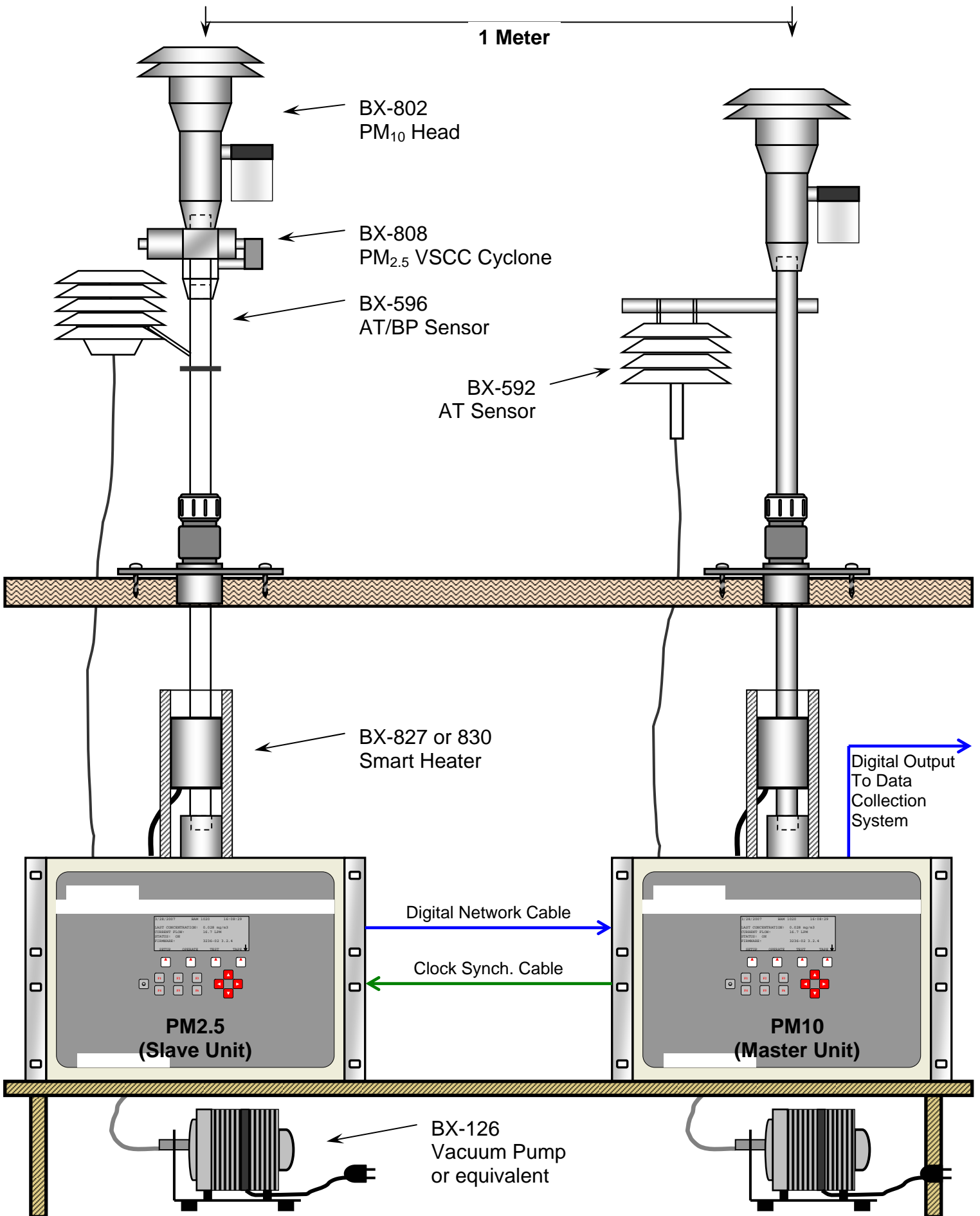
Figure 1: BAM-1020 PM-Coarse System
